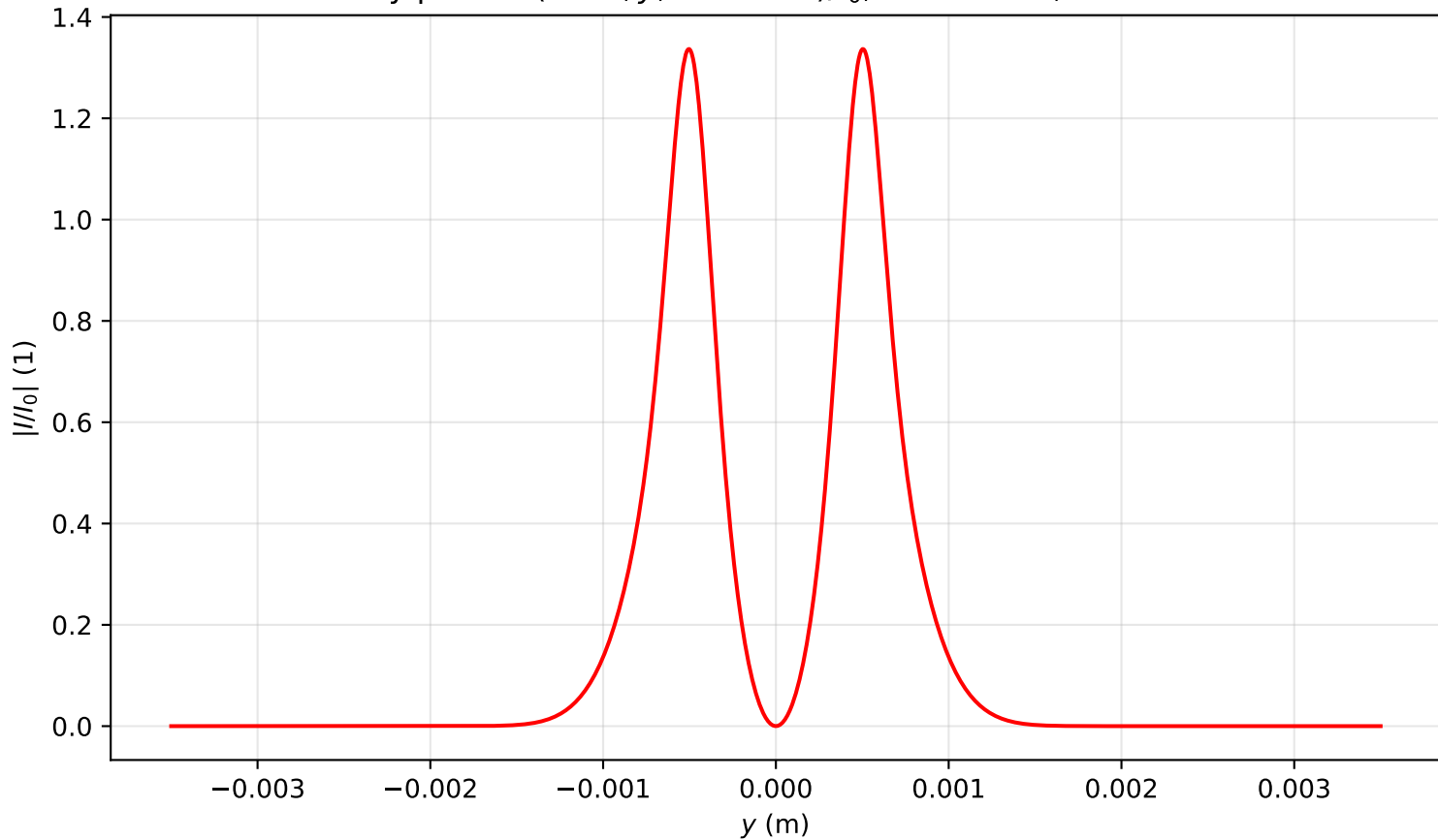
Intensity profile I(x=0, y, z=0.318)/I_0 , \text{Pin}=8.0\text{Pcr} , artificial time
